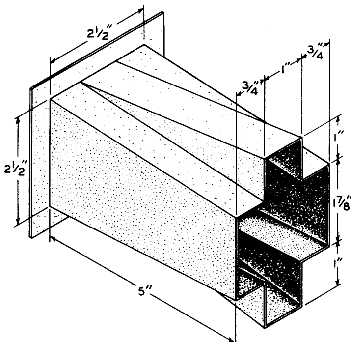
AIR DUCT
