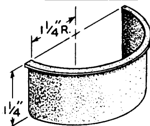
AIR DEFLECTOR
